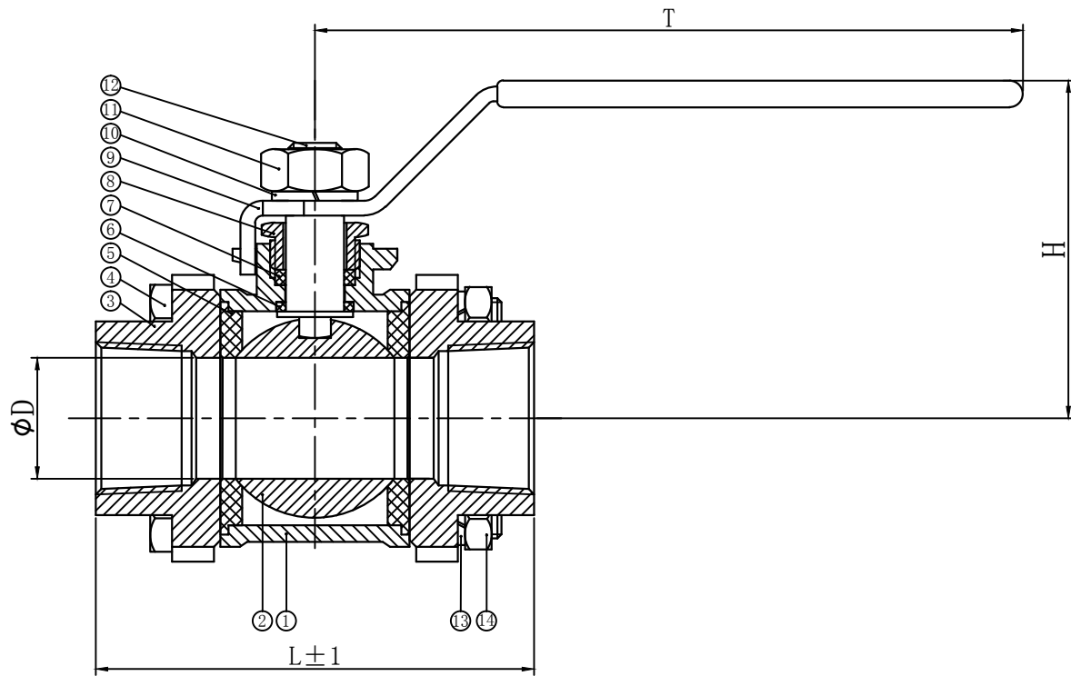
CONFIGURATION DIMENSION
